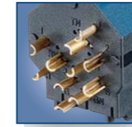
Solder termination
