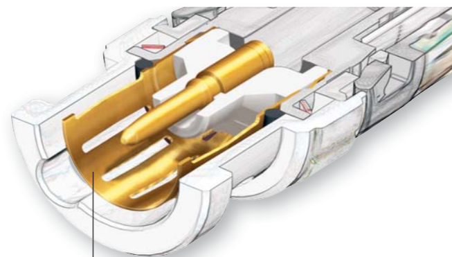
Gold plated ground contact with improved shielding effectiveness optimized for high frequency HDTV signal up to 3 GHz.
