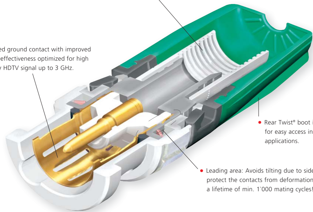
Neutrik BNC: no tilting due to side pull
